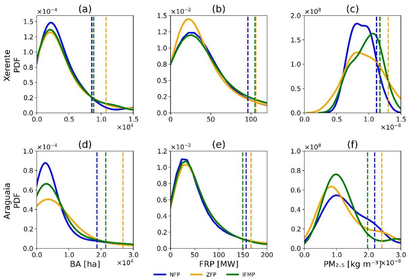
Figure 4. Kernel Probability density function (PDF) of burned area (BA, ha) for large scars (a,d), Fire Radiative Power (FRP, MW, b,e) and pyrogenic emission ( PM_{2.5} , kg\ m^{-3} , c,f) for WFS during each phase (NFP—blue, ZFP—yellow, IFMP—green) for in the Xerente (upper row) and Araguaia (bottom row). The dashed lines represent the 90th percentile for each respective phase.
