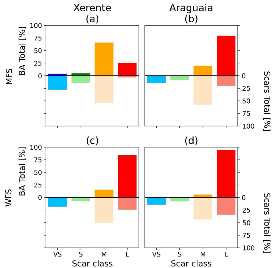
Figure 2. Total burned area (BA, %, full color) and scars (%; smoothed color) per scar size class: very small (VS, blue), small (S, green), medium (M, orange), and large (L, red) in the management fire season (MFS, upper row) and wildfire season (WFS, bottom row) from 2003 to 2018 in Xerente (a,c) and Araguaia (b,d).
