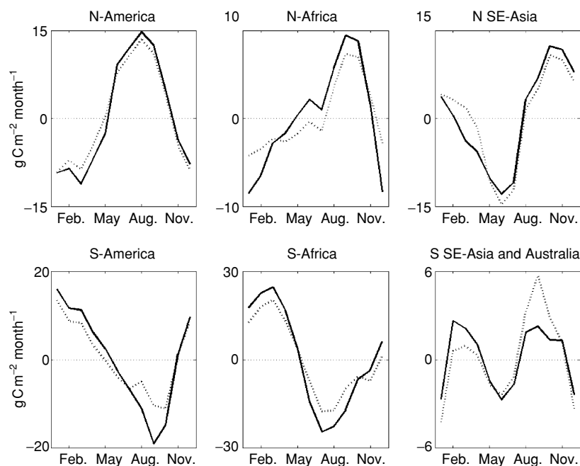
Fig. 10 Seasonal net biome production for model runs with (solid line) and without (dashed line) fire influences. Positive values represent a flux towards the biosphere, negative towards the atmosphere.
