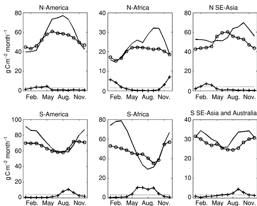
Fig. 9 Seasonal carbon fluxes for different regions. The solid line represents NPP, the circled line microbial respiration, pluses direct fire emissions, and the dashed line the sum of herbivore heterotrophic respiration and fuel wood consumption. Northern regions are defined as all areas north of the equator.
