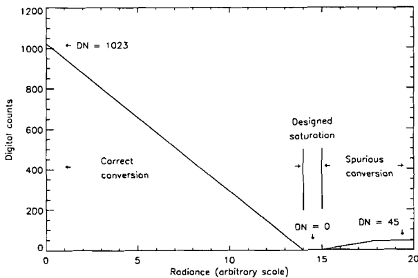
Figure 3.1 Possible explanation for the nonsaturation of channel 3 by fires and highly reflective targets, due to a spurious signal conversion (after Setzer and Verstraete 1993)
