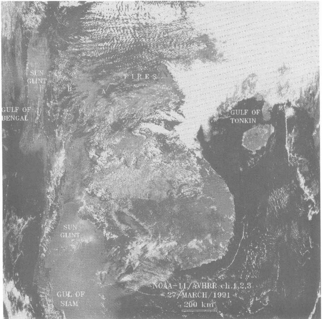
Figure 3.5 The NOAA-11 AVHRR image of Southeast Asia on 27 March 1991 showing major fire activity in its upper part. Strong ocean sunglint occurs in the Gulf of Siam, and land reflection is found east of the Gulf of Bengal. Fires A and B at the origin of large smoke plumes are described in the text.
