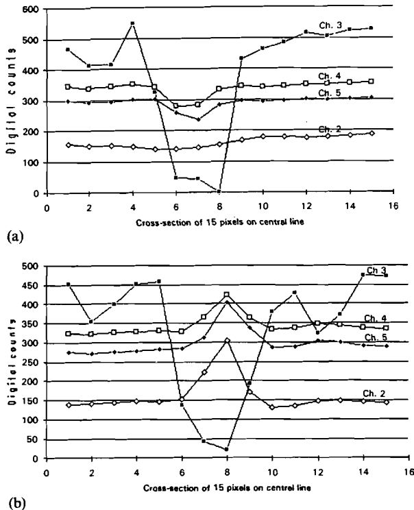
Figure 3.2 The DN cross-section through two fires in AVHRR channels 2–5. In (a) channels 3, 4, and 5 respond similarly to the fire, but in (b) the response of channels 4 and 5 is inverse. See figure 3.5 for the location of the two fires.
