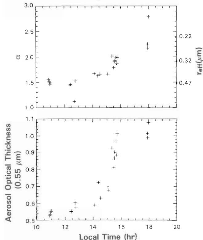
Fig. 10. Sunphotometer observations made during September 3 and 4, 1989, of the optical thickness ( \tau ) for (bottom) 0.55 \mu\text{m} and (top) its spectral dependence ( \alpha ) for background mixed smoke conditions as a function of the time of the day. The corresponding effective particle radius ( r_{\text{eff}} ) is also given.
