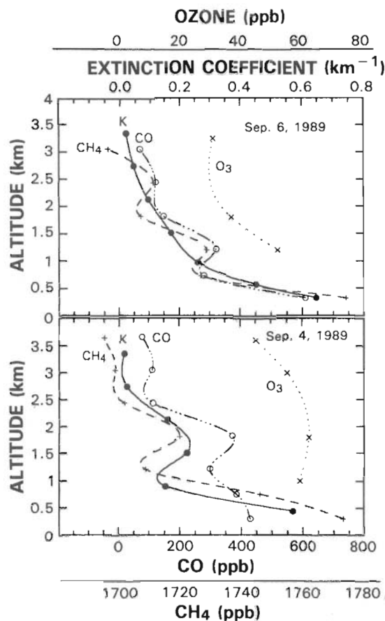
Fig. 4. Profiles of the CO (open circles), CH 4 (pluses), and ozone (crosses) concentrations and simultaneous extinction coefficient (solid circles) profiles at 0.45 \mu\text{m} (an optical measurement proportional to the particulate matter concentration). September 6, 1989, at 0830–0930 LST and September 4, 1989, at 1100–1200 LST.
